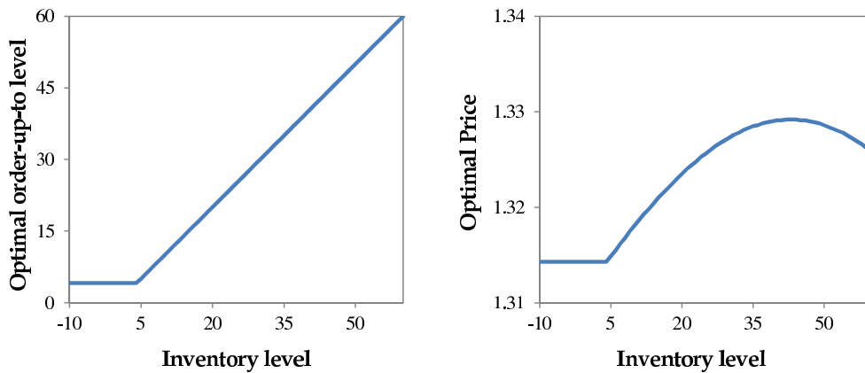
Figure 1 An example in which the optimal price is not monotone in the inventory level.
